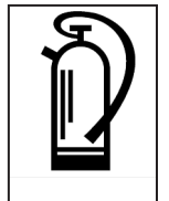
Carbon dioxide CO 2
